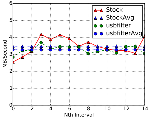
Figure 7: Iperf bandwidth ( MB/s ) using UDP with different time intervals.
